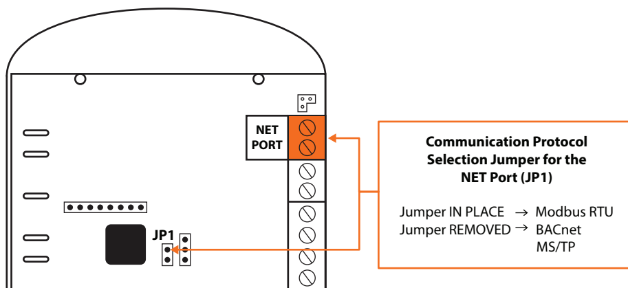
Figure 16 - Communication Protocol of the NET Port
