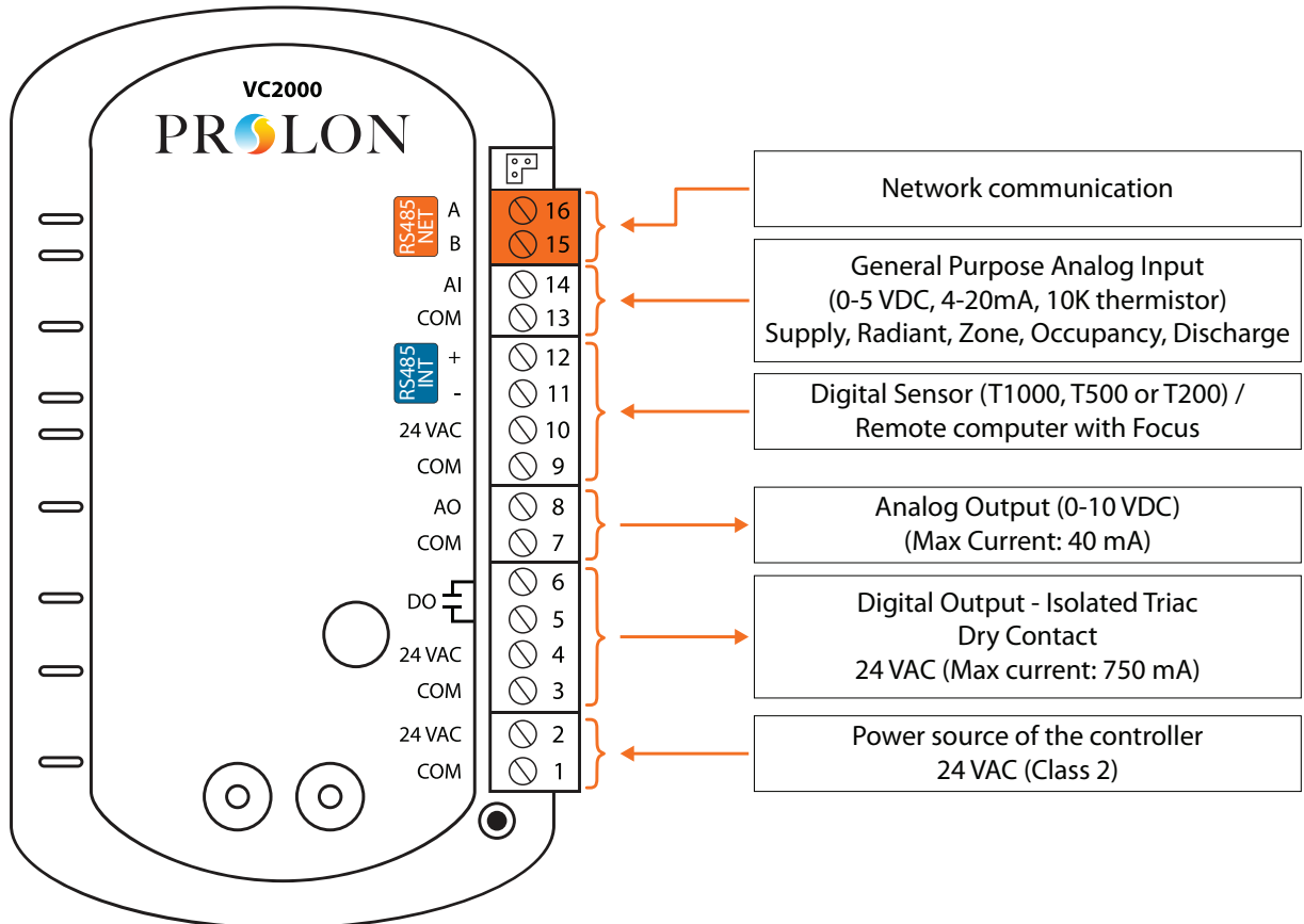
Figure 2 - Terminal Block Identification
