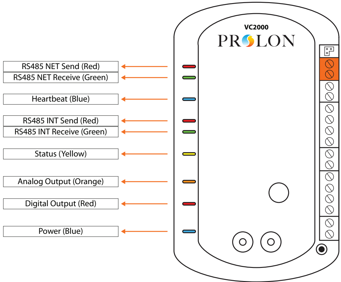
Figure 3 - LED Identification
